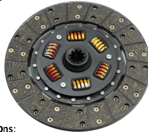
3210315AF – 232mm/91/8” dia. D.P. Assembly
